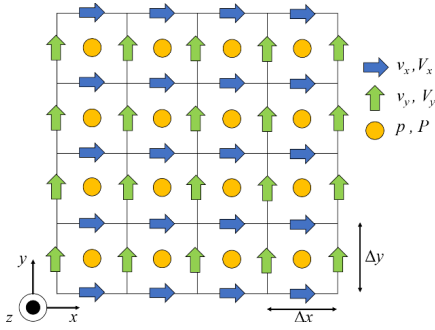
Fig. 1 Yee grid for finite difference scheme for space discretization. \Delta x and \Delta y are the segmented areas. The particle velocity vector and the sound pressure are discretized by half-cell displacement.
