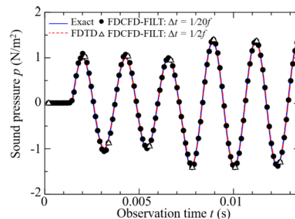
Fig. 5 Time response of sound pressure at the observation point. The exact solution, FDTD results, and results obtained using the proposed method are in agreements. Arbitrary time step size can be selected in the proposed method.
