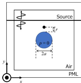
Fig. 3 Computational model for validation of the proposed method. The scatterer is a cylinder of radius a and consists of acoustic soft medium ( p = 0 at the boundary).
