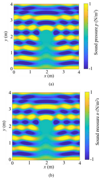
Fig. 4 Sound pressure distribution over the computational area. (a) FDTD and (b) FDCFD-FILT. Observation time t = 0.0135 s. FDCFD-FILT can compute the sound field at specific observation time.
